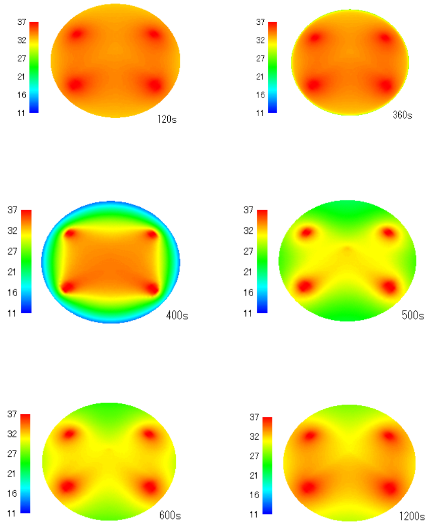
Fig. 3 Isotherm contours of the finger in different time
