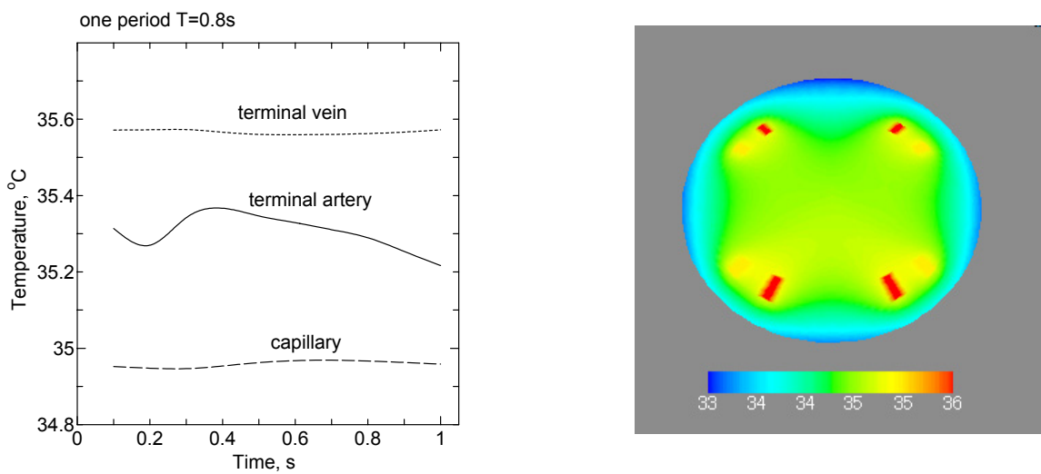
Fig. 12 (a) Blood Temperatures in Artery, Vein, Capillary (b) Blood Temperature in Solid Tissues of Modeled Finger
